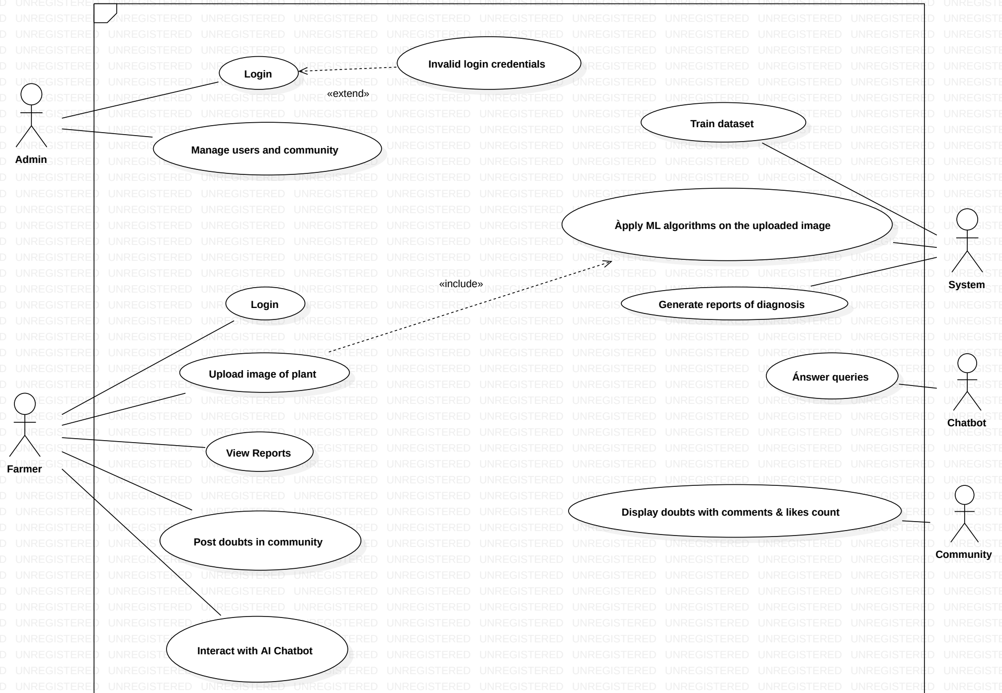
Model2::AgrismartUseCaseDiag
